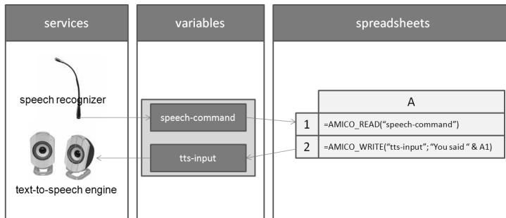
Fig. 3. An example of the communication among diverse elements of Sketchify through variables. In this example, a speech recognizer updates the variable “speech-command” with the recognized word. Within a spreadsheet, this variable is read, and the variable “tts-input” is updated in response. Update of this latter variable is propagated to a text-to-speech engine that pronounces the given text.
