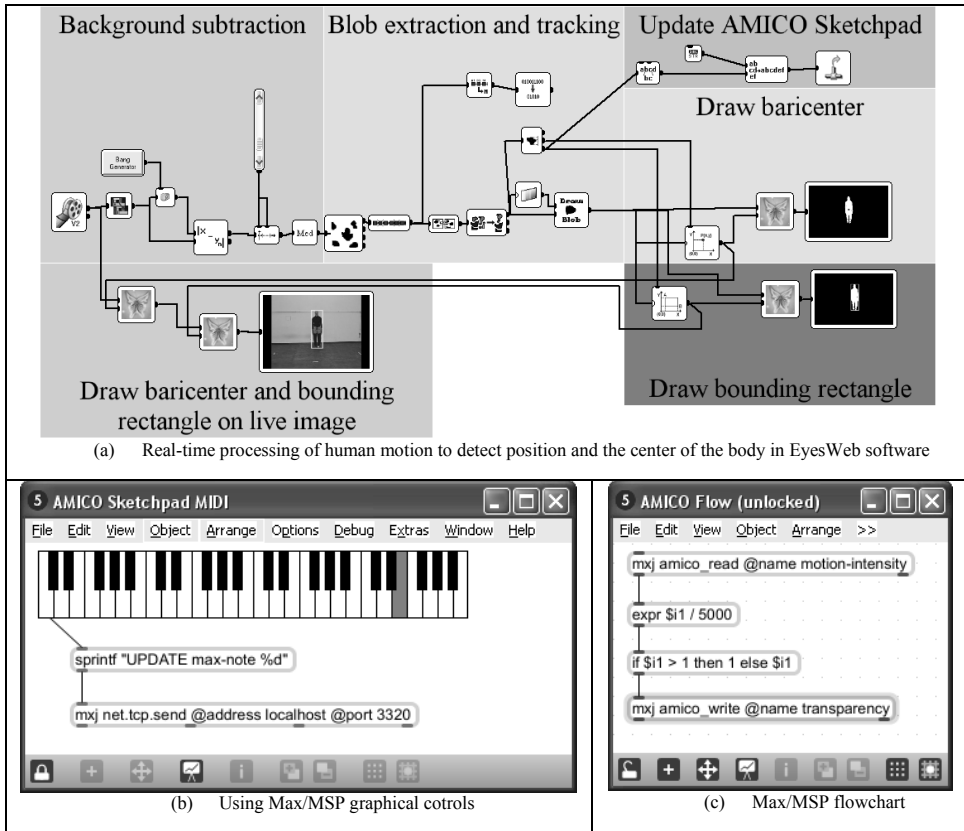
Fig. 4. Connecting the EyesWeb (a) and Max/MSP (b) and (c) environments with Sketchify.
