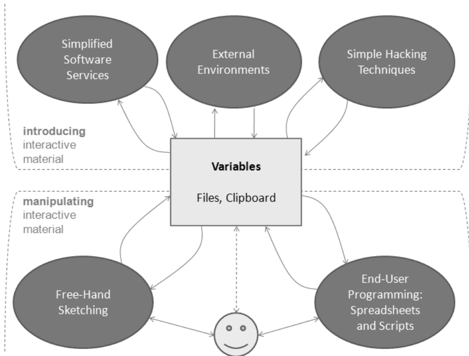
Fig. 2. Sketchify combines free-hand sketching with support for state transitions and animation, end-user programming, and I/O services. Sketchify also offers the possibility to exchange information with existing software environments and simple hacking techniques. Blackboard architecture of globally available variables is used to connect all elements.
