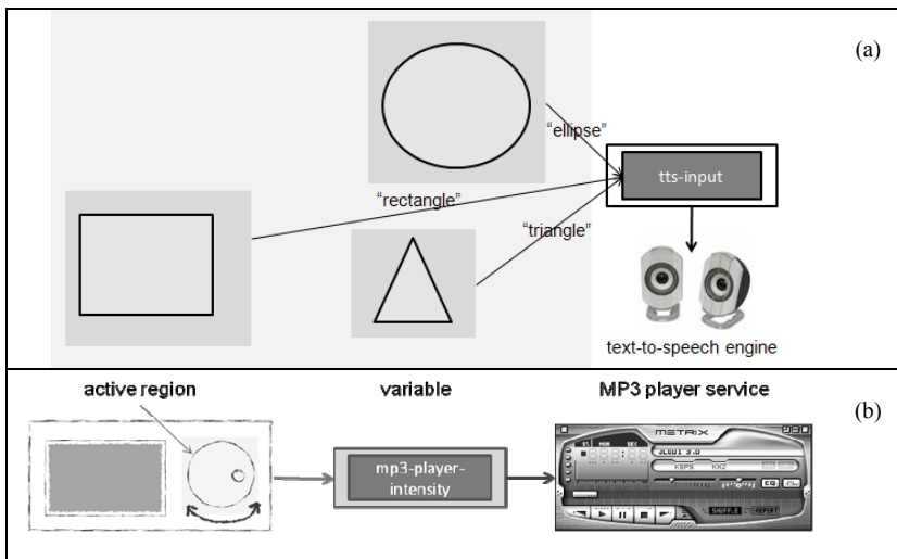
Fig. 9. Mapping mouse button clicks (a) and mouse movements (b) to variable updates that trigger interactive events, in this case output of the text-to-speech service, and changing the volume of the MP3 player.
